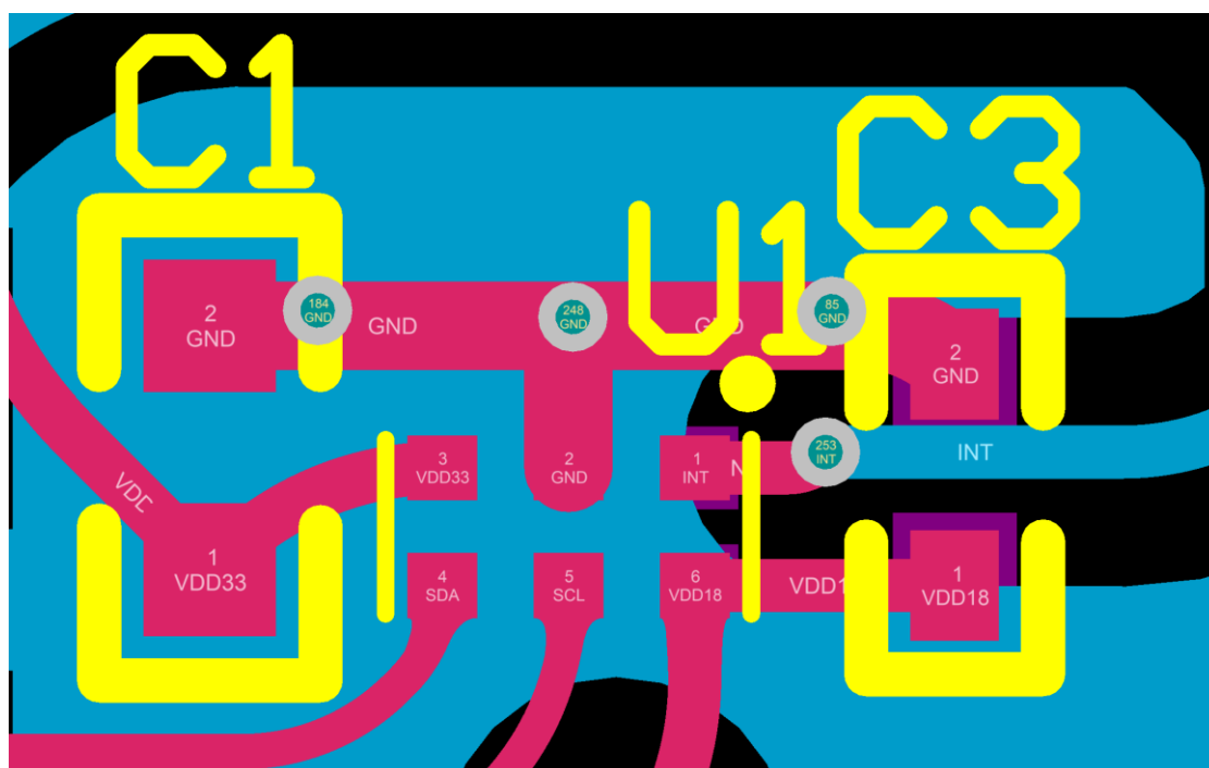
Recommended Circuit Layout
